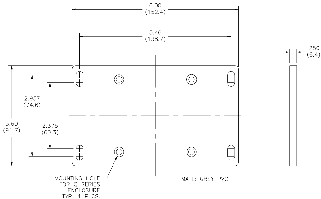
Figure 3 - Wall or Pipe mount Bracket
