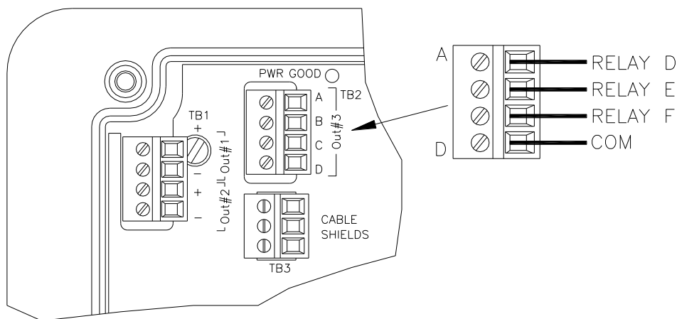
Figure 12 - Low Power Relay Connections
