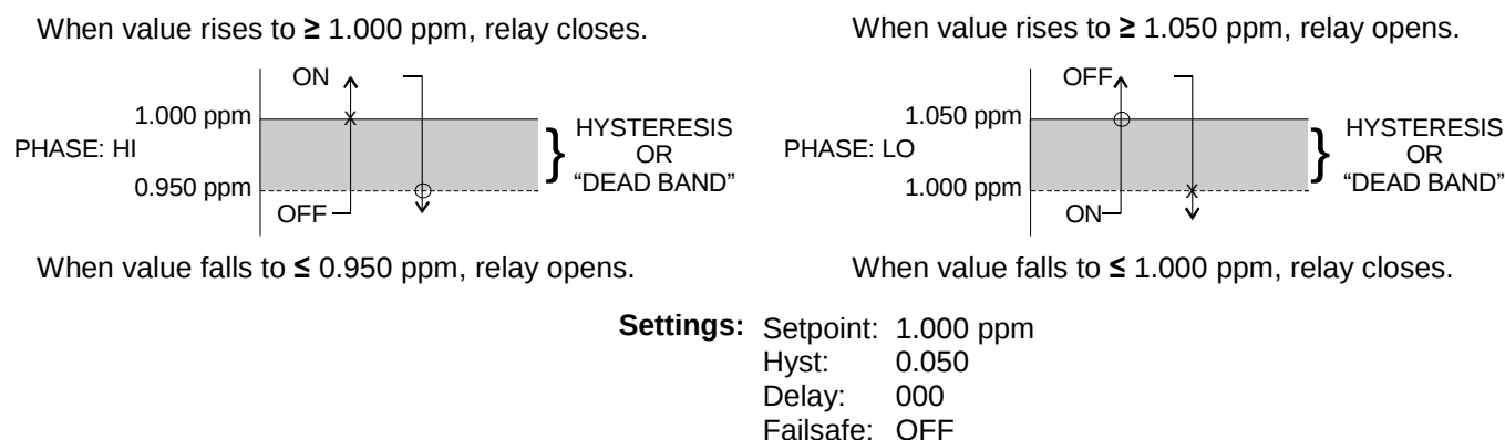
Figure 15 - Control Relay Example
