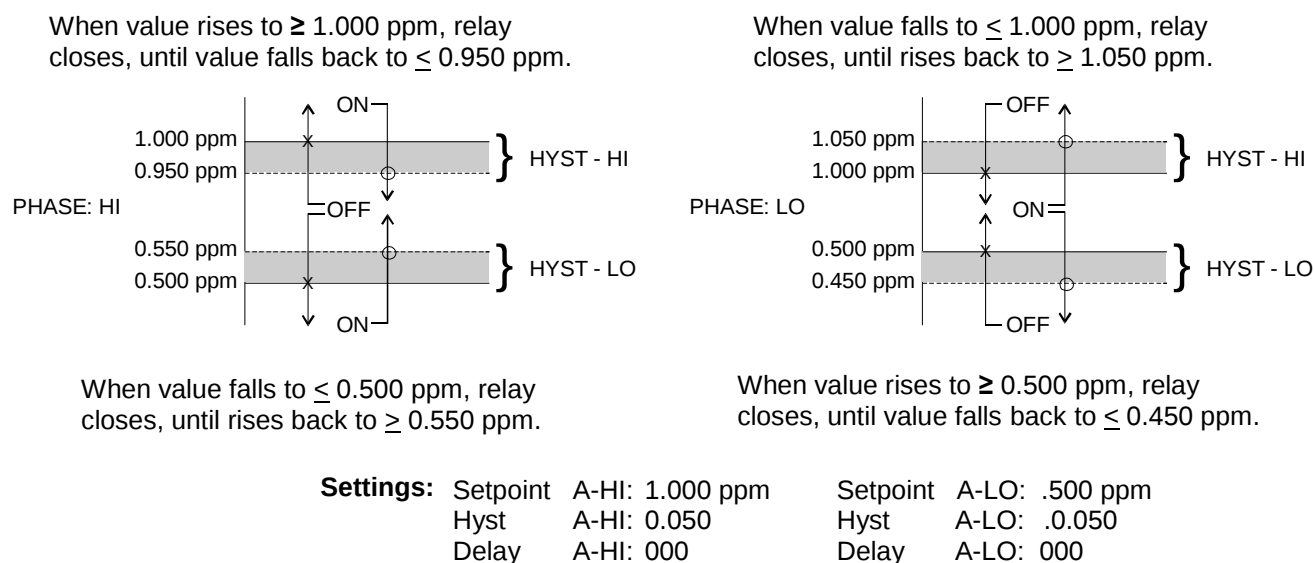
Figure 16 - Alarm Relay Example
