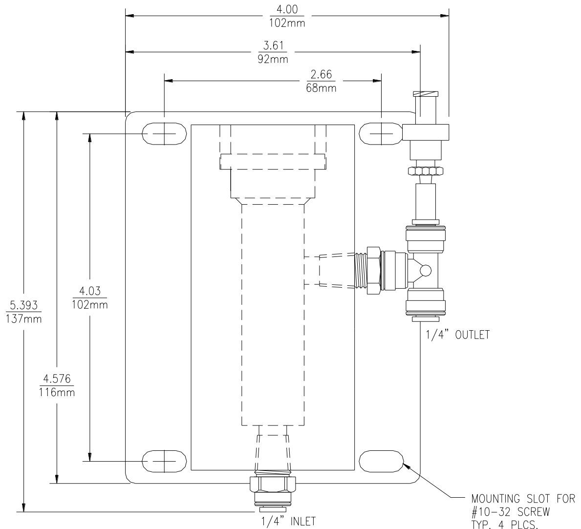
Figure 7 - Fluoride Flowcell
