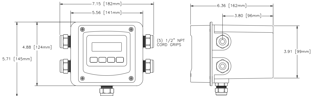
Figure 2 - Q46F Enclosure Dimensions
